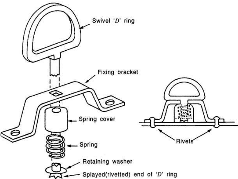
Fig 6 Example of Swivel Ring l'D' Ring
