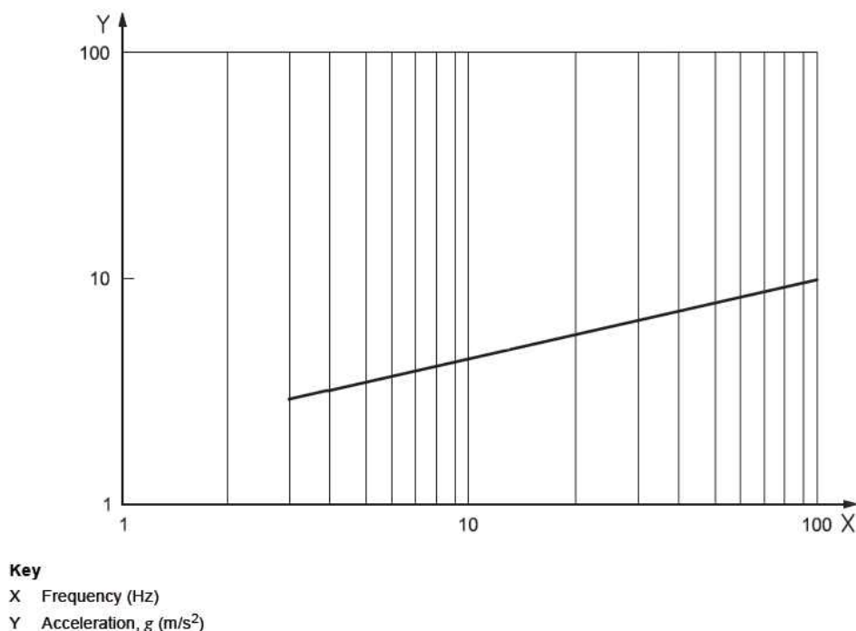
Fig 2.23 Minimum SRS Curve (5 % Damping)
